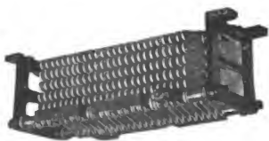
Fig. 4663. Grid Resistance. Westinghouse A. C. Electric Locomotive.
